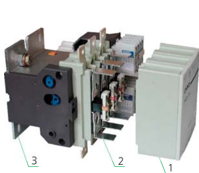
1: arc-extinguishing system
