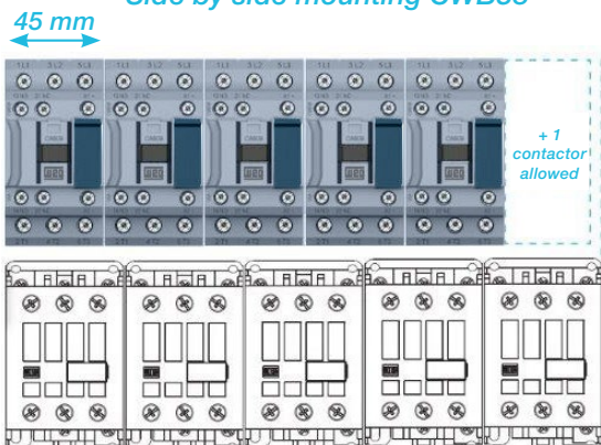
Side by side mounting CWB38
