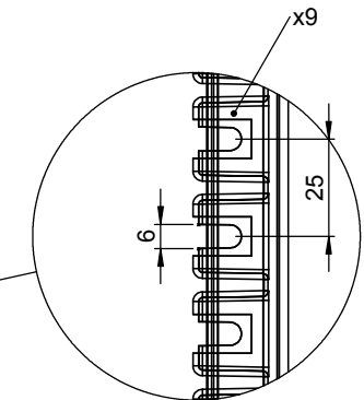
DETAIL C
