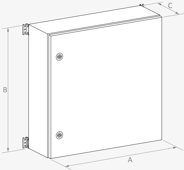
WALL MOUNTING
