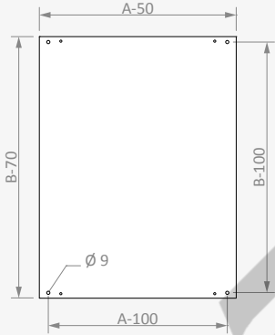
MOUNTING PLATE
